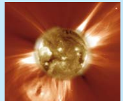
Sun Storm: A Coronal Mass Ejection © SOHO Consortium, ESA/NASA
